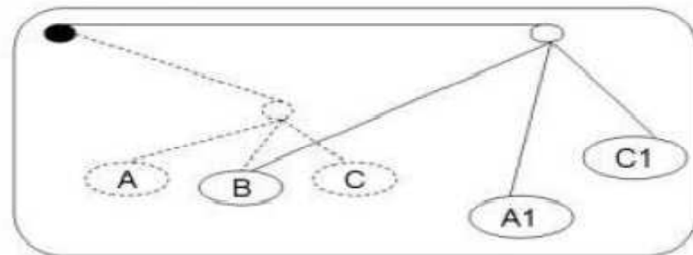
Database Version 2
