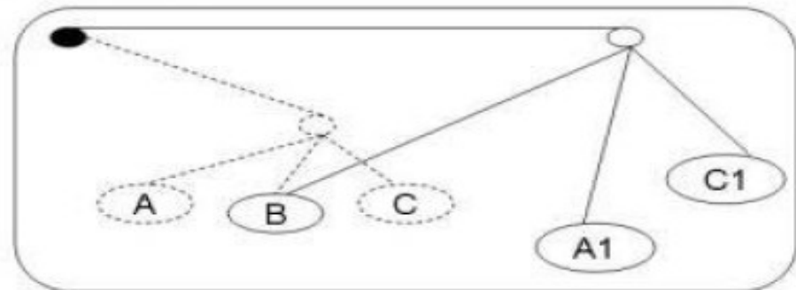
Database Version 2
