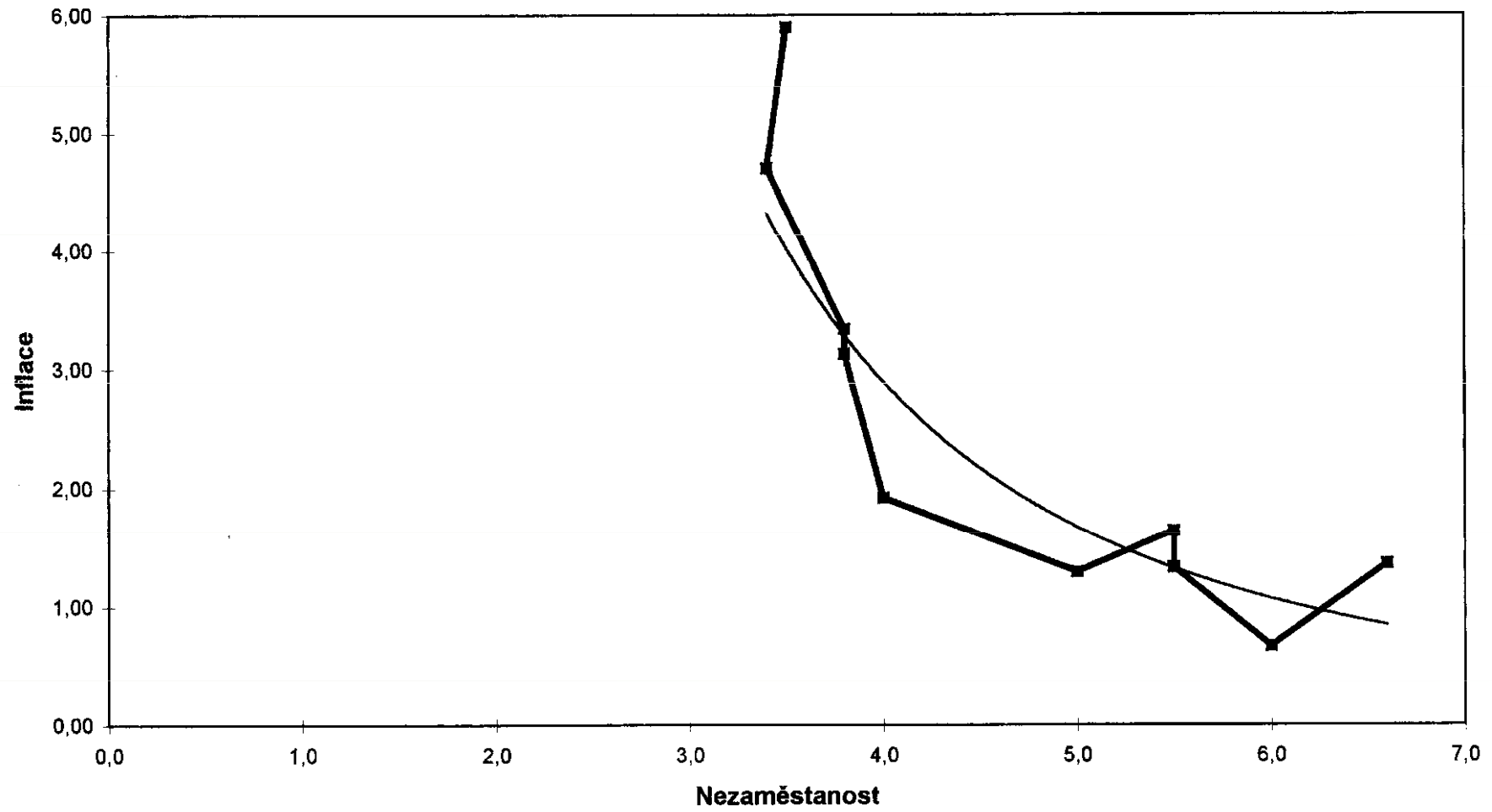
Phillipsova křivka 1960 -1969
