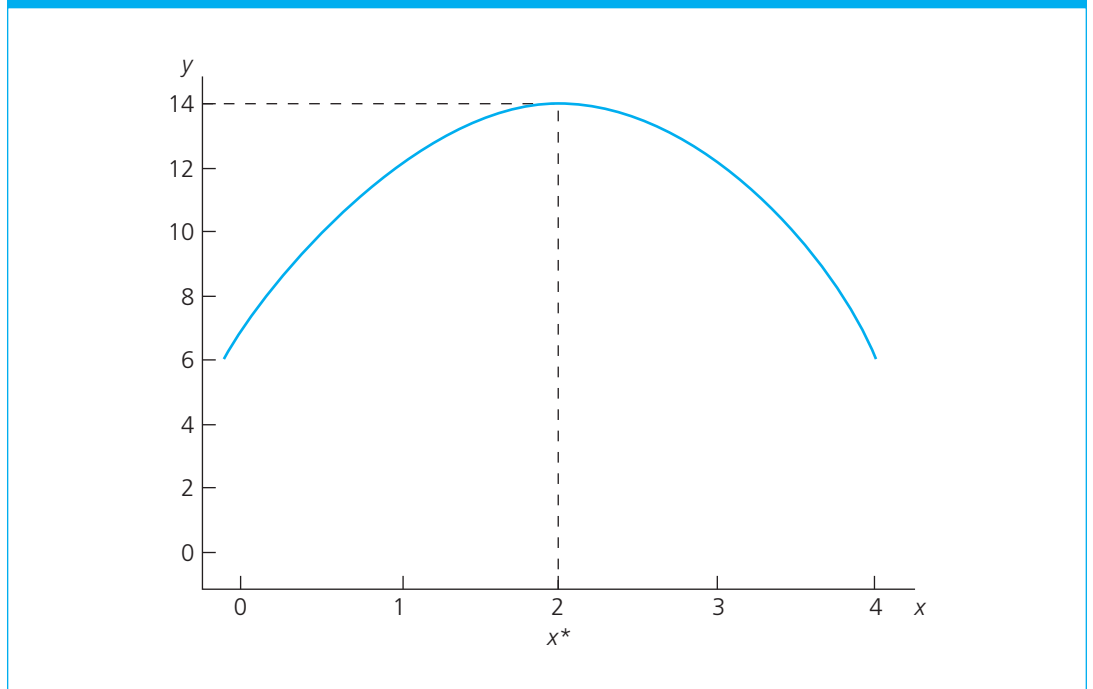
FIGURE A.3 Graph of y = 6 + 8x - 2x^2 .
