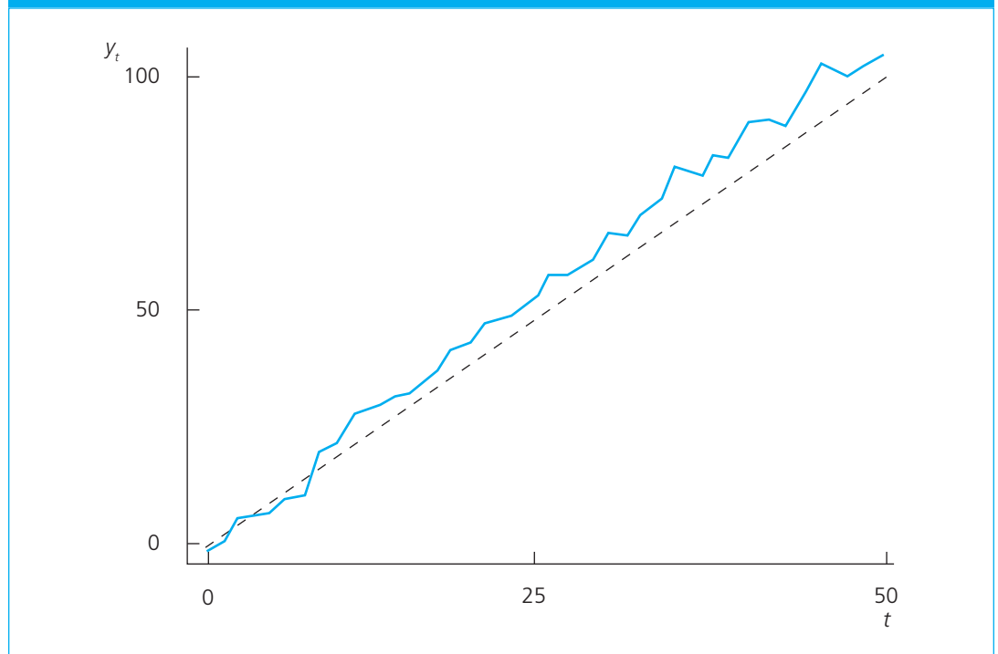
FIGURE 11.3 A realization of the random walk with drift, y_t = 2 + y_{t-1} + e_t , with y_0 = 0 , e_t s Normal(0, 9), and n = 50 . The dashed line is the expected value of y_t , E(y_t) = 2t .
