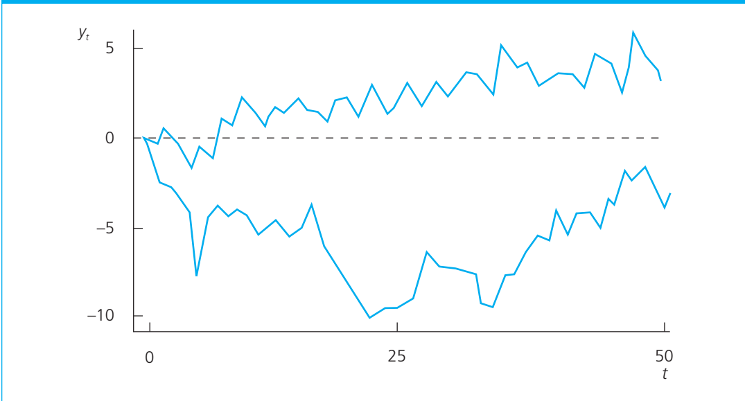
FIGURE 11.1 Two realizations of the random walk y_t = y_{t-1} + e_t , with y_0 = 0 , e_t \sim \text{Normal}(0, 1) , and n = 50 .
