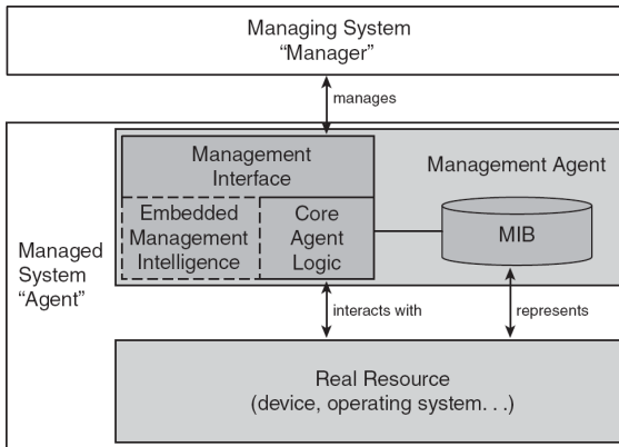
Figure: Anatomy of a Management Agent.
