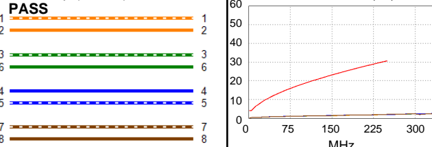
Wire Map (T568B)
