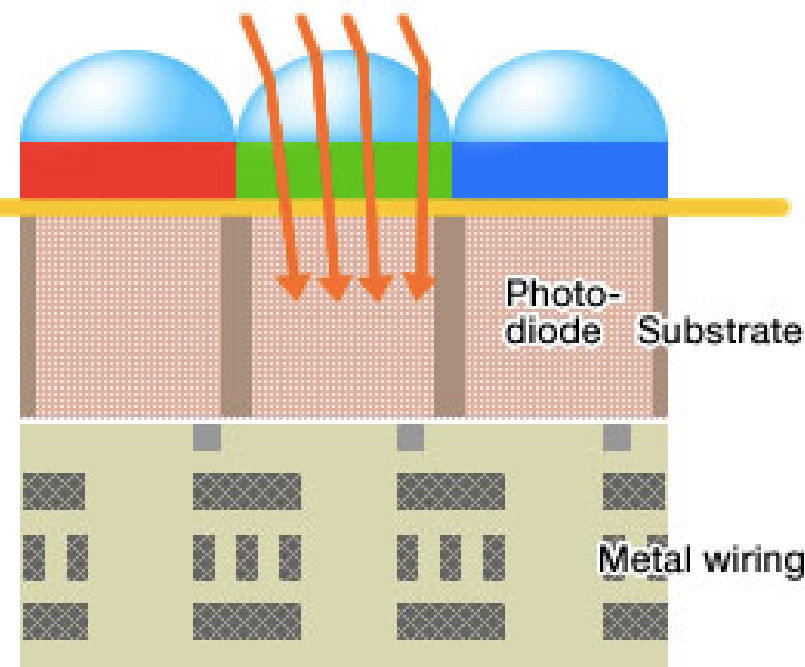
back-illuminated structure
