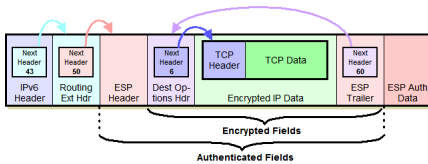
IPv6 ESP Datagram Format - IPsec Transport Mode
