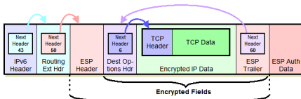
Authenticated Fields IPv6 ESP Datagram Format - IPsec Transport Mode
