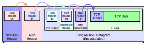
IPv6 AH Datagram Format - IPsec Transport Mode
