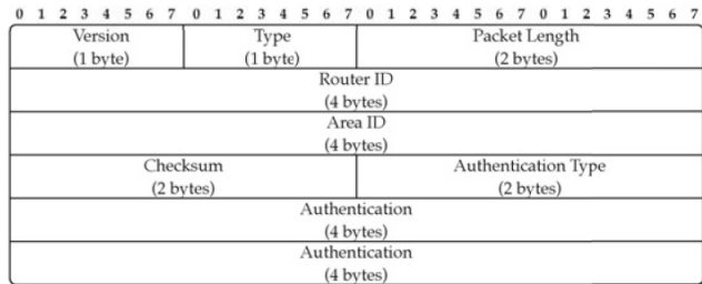
Figure: OSPF packet common header.
