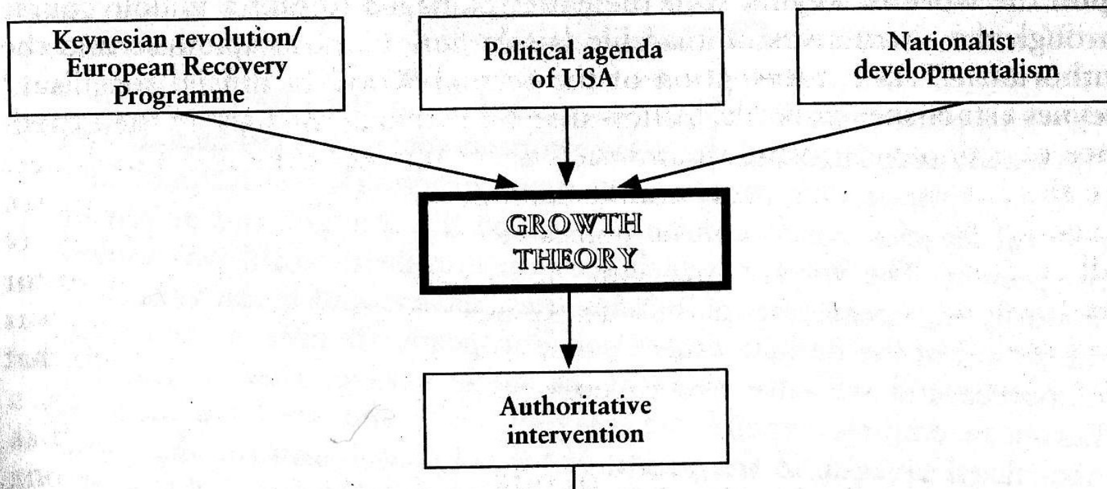
Figure 10 Growth theory
