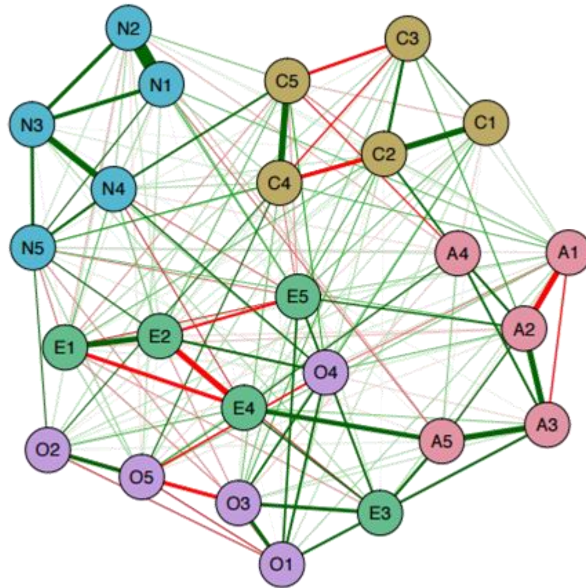
Figure 1.1: Example of a network model estimated the BFI personality dataset from the psych package in R. Nodes represent variables (in this case, personality inventory items) and links between the nodes (also termed edges ) represent partial correlation coefficients. Green edges indicate positive partial correlations, red
