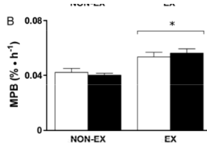
FIGURE 4 —Mixed muscle protein fractional synthetic rate (MPS) and breakdown rate (MPB). *Significant main effect of exercised (EX) versus nonexercised (NON-EX; P < 0.05 ). The dashed line on the upper graph indicates a mean resting and fasted rate of MPS obtained from previous studies (6,24,30,31) of 0.041\% \cdot h^{-1} \pm 0.006\% \cdot h^{-1} to illustrate differences from the rested fasted state. Values are means \pm SEM.
