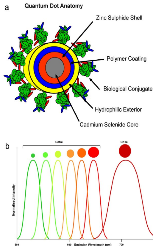
Figure 1. (a) Schematic representation of a QD Quantum dots are composed of a Cadmium Selenide (CdSe) core, around which a Zinc Sulphide (ZnS) shell is added to increase quantum yield. Addition of polymer and hydrophilic coverings is required for stability and the outside of the assembly is coated with biomolecules such as streptavidin or amine to enable attachment to other molecules (reproduced with permission from Tholouli et al , J Pathol 2008, 216, 275-285).
