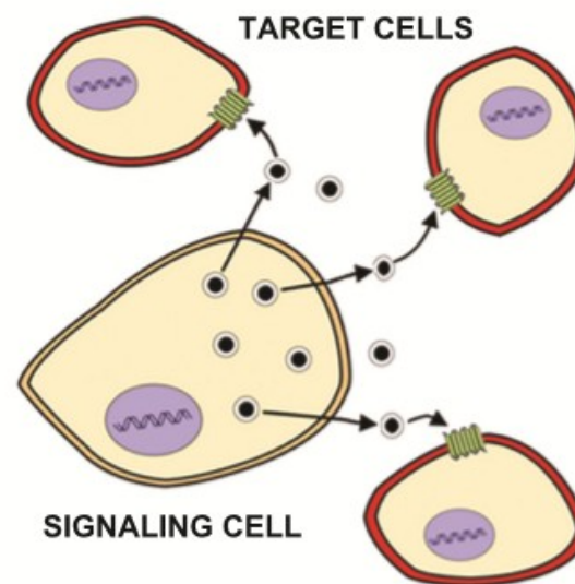
3. PARACRINE
