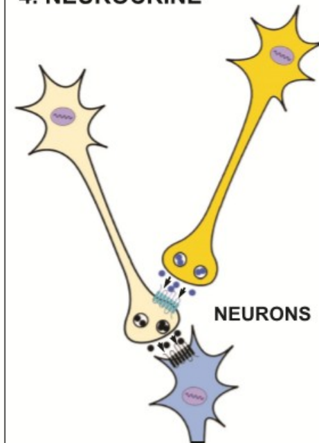
4. NEUROCRINE
