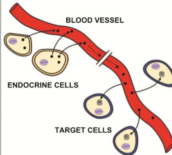
5. ENDOCRINE
