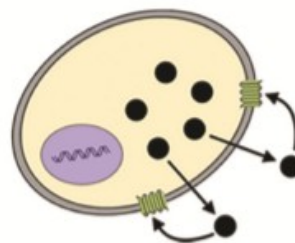
2. AUTOCRINE
