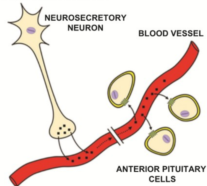
6. NEUROENDOCRINE
