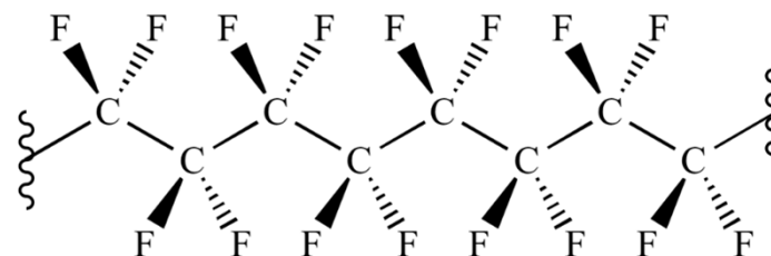
PTFE (Teflon)
