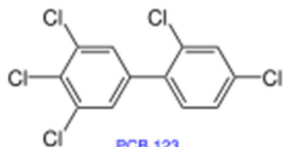
PCB 123
