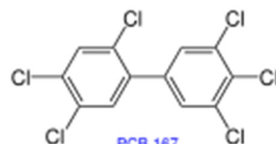
PCB 167
