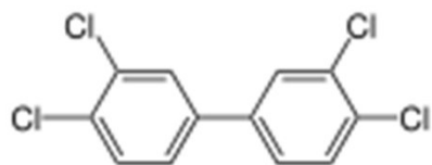
PCB 77
