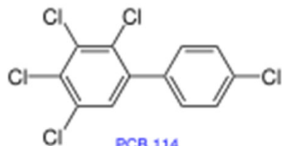
PCB 114
