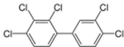
PCB 105
