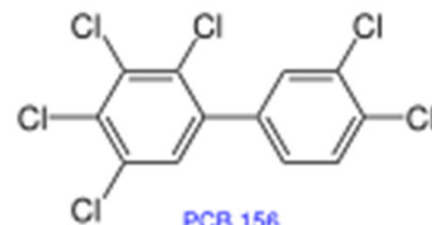
PCB 156
