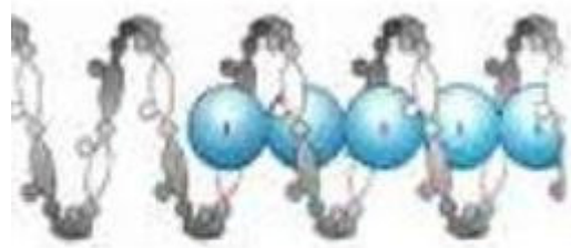
Amylose-iodine complex
