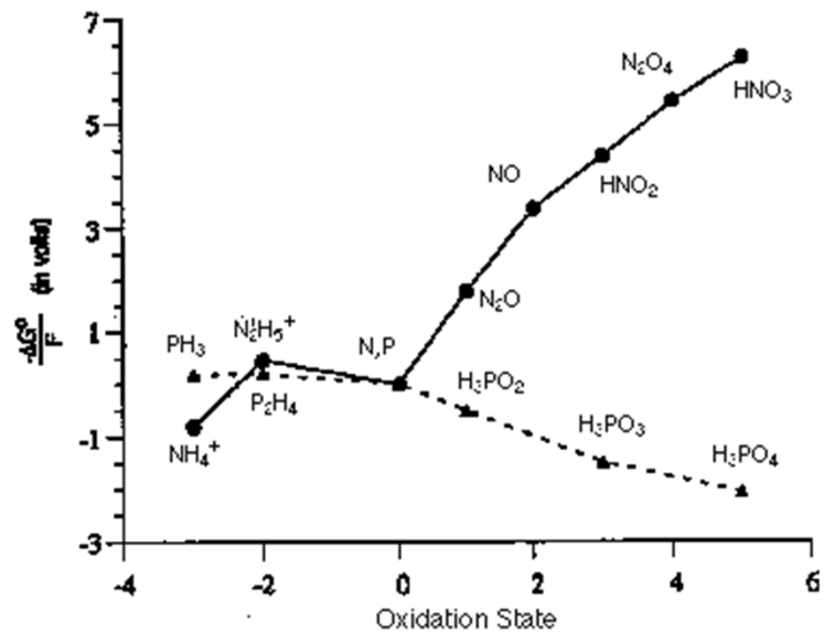
Fig. 8.4 Frost–Ebsworth diagrams in aqueous solution at pH 0, i.e. [\text{H}^+] = 1 \text{ mol dm}^{-3} , for (b) phosphorus
