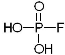
fluorophosphoric acid
