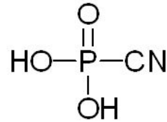
cyanophosphoric acid
