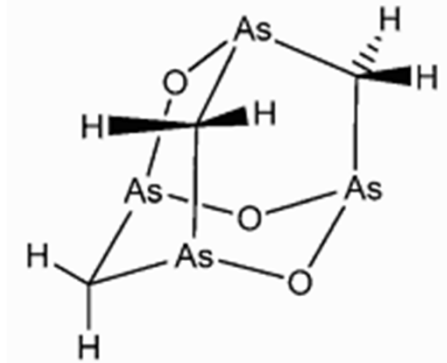
Arsenicin A
