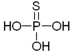
thiophosphoric acid
