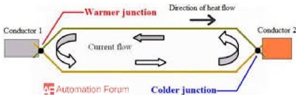
Peltier Effect
