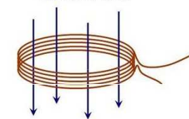
Flux linkage of a coil = N \times \Phi = N \times B \times A
