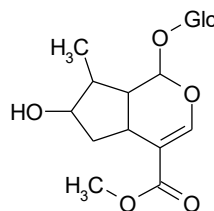
loganin
