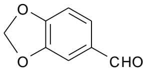
piperonal (= heliotropin)
