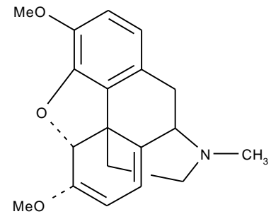
thebain
