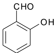
salicylaldehyd
