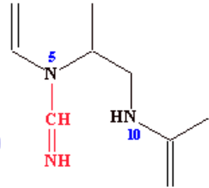
N 5 -Formimino-tetrahydrofolate carries methenyl groups
