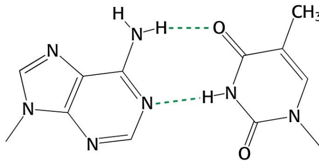
Adenine
