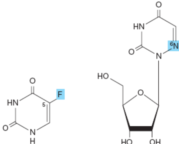
5-Fluorouracil
