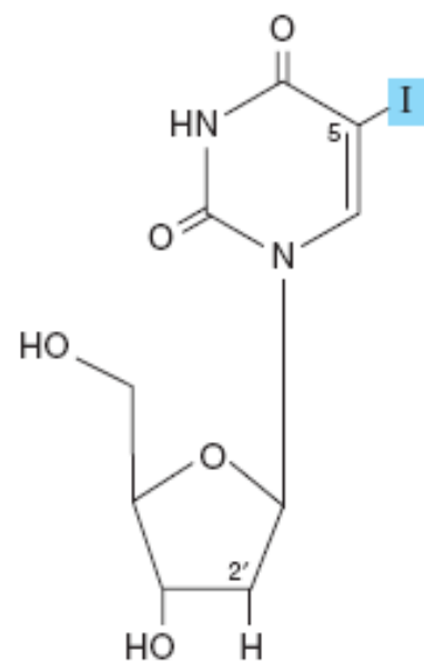
5-Iodo-2'-deoxyuridine
