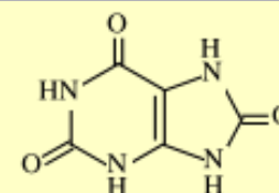
Uric acid
