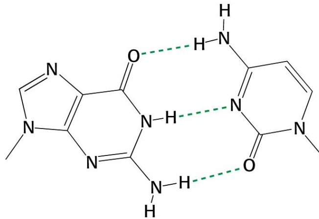
Guanine
