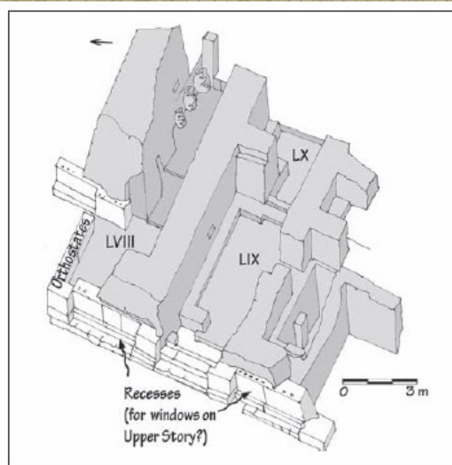
5.3. Reconstruction. West wing, Palace at Phaistos. After Levi 1976, pl. N.
