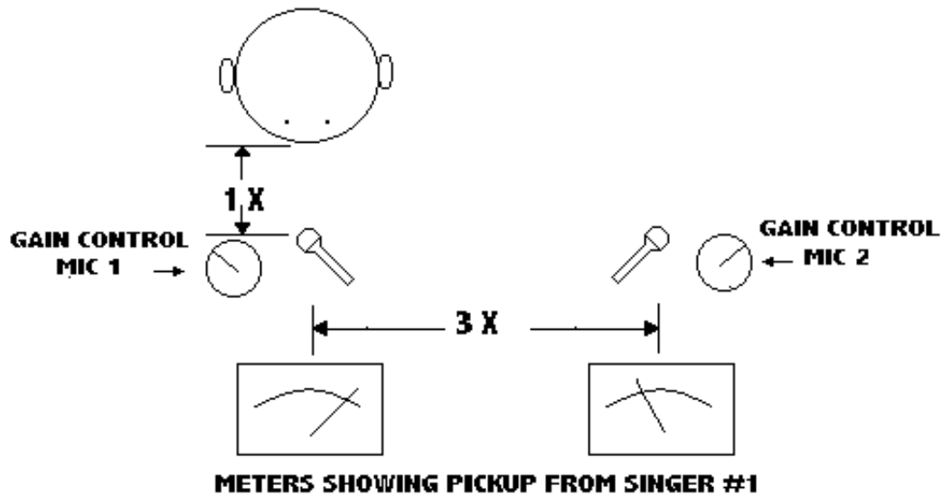
FIGURE 9 - STRONG & WEAK SINGER USING 3 TO 1 PLACEMENT AND CARDIOID MICS
