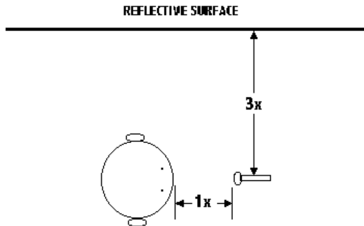
FIGURE 11 - USING 3 TO 1 TO PREVENT REFLECTIVE PHASE CANCELLATION
