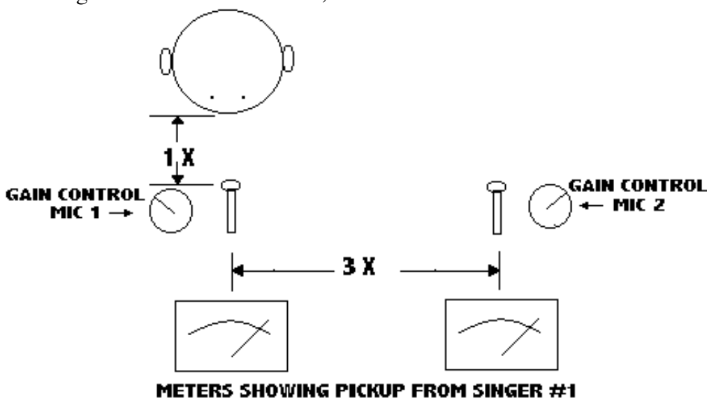
FIGURE 5 - STRONG & WEAK SINGER USING 3 TO 1 PLACEMENT
