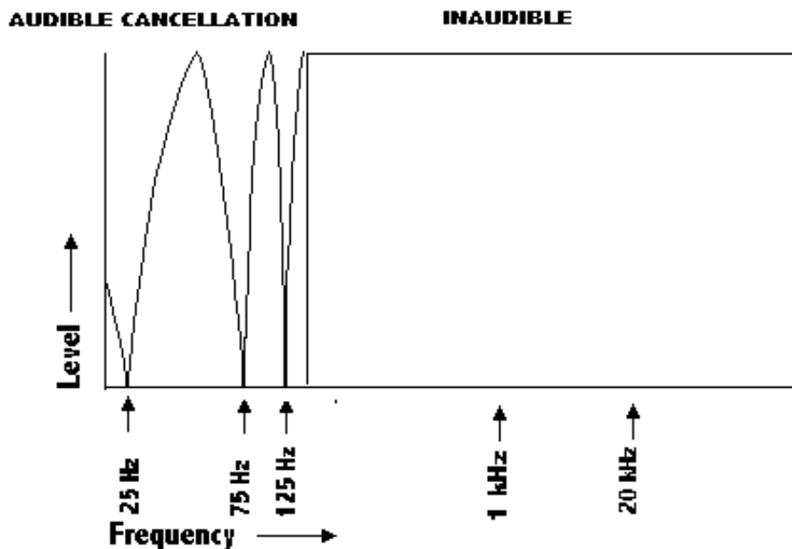
FIGURE 13 - FREQUENCIES CANCELING WITH 20 MS DELAY BETWEEN MICS
