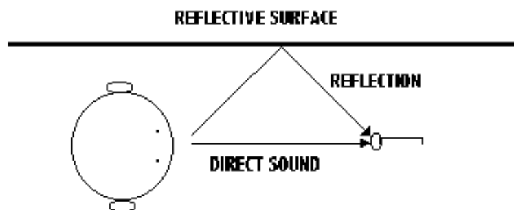
FIGURE 10 - REFLECTION CAUSING PHASE CANCELLATION
