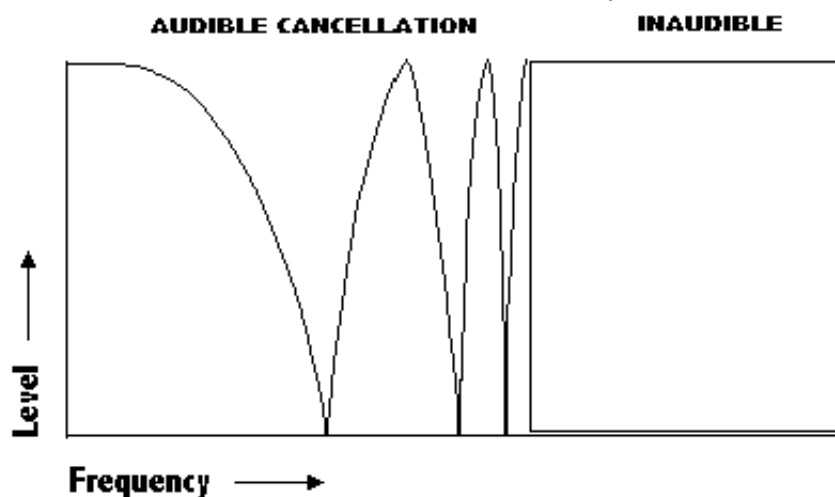
FIGURE 2 - COMB FILTER
