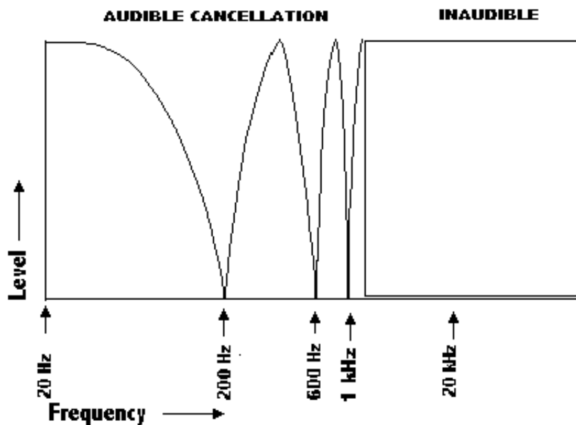
FIGURE 12 - FREQUENCIES CANCELING WITH 2.5 MS DELAY BETWEEN MICS
