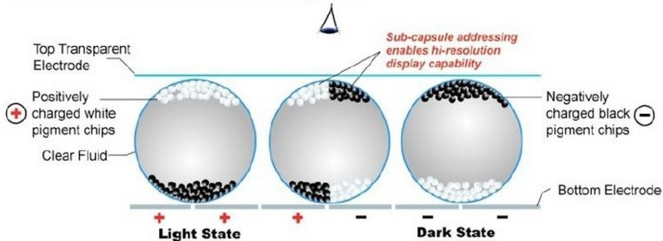
Cross-Section of Electronic-Ink Microcapsules
