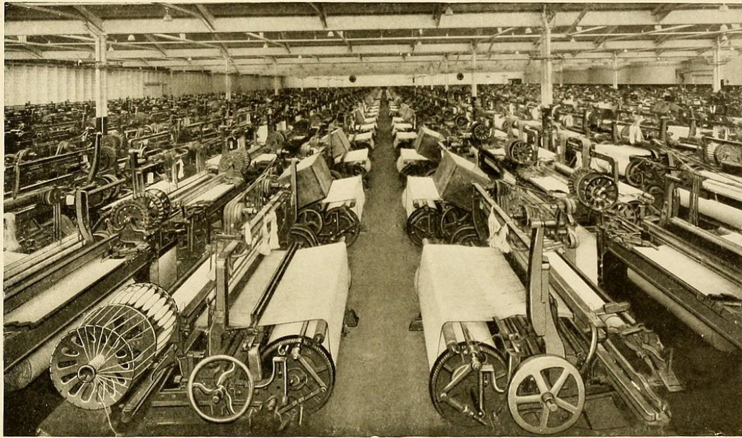
INTERIOR VIEW OF A MODERN WEAVE-ROOM (Courtesy of the Chicopee Manufacturing Company)
