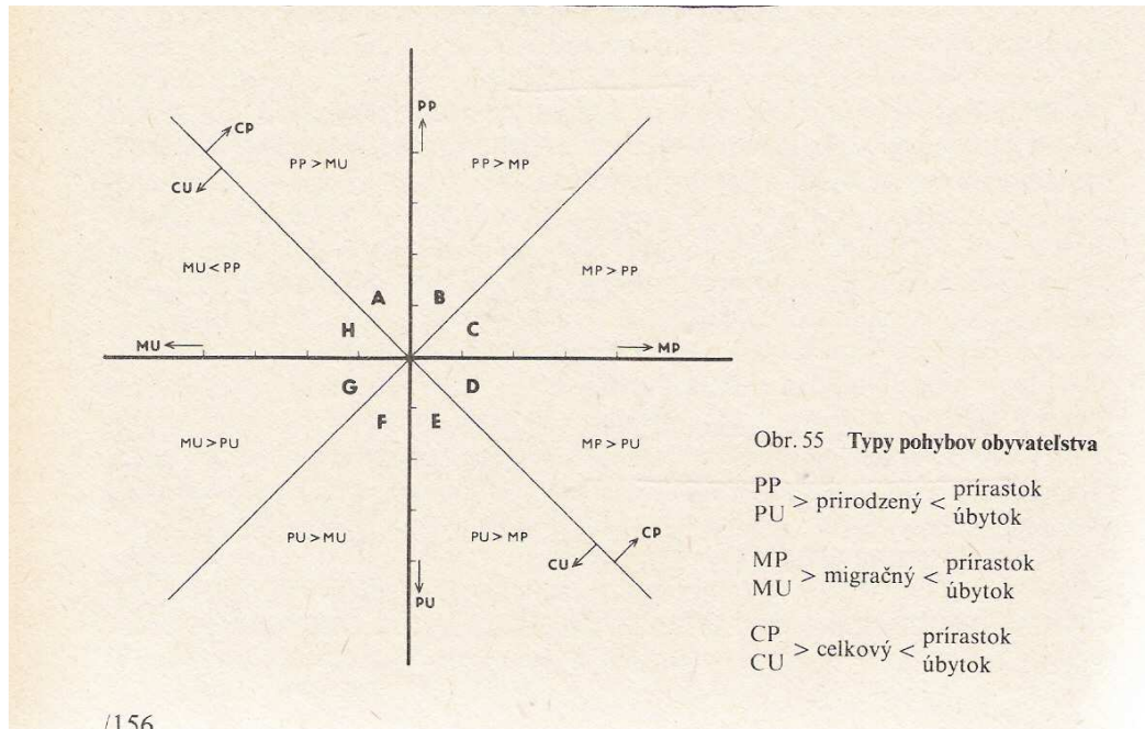
Obr. 5: Webbův diagram
