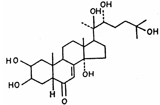
20-Hydroxyecdysone
