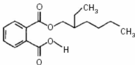
Mono-(2-ethylhexyl) (MEHP)
