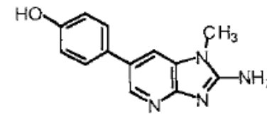
4'-hydroxy-PhIP
