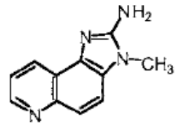
IQ
