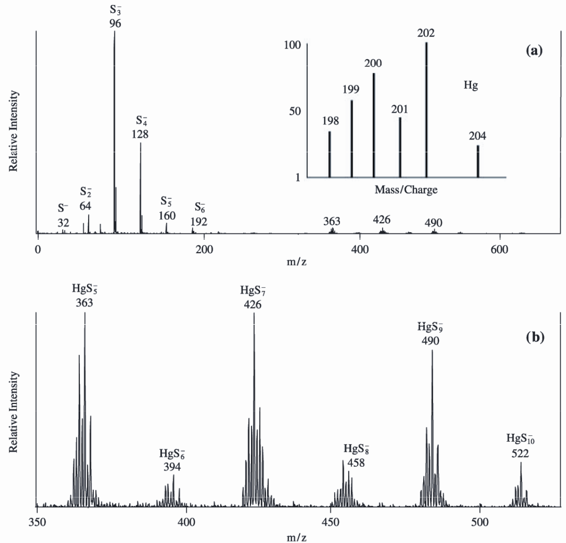
Figure 5 (a) A negative ion LDMS spectrum of the red ink/dye region of the Qur'an sample. (b) An expanded view of the higher m/z portion of the spectrum.
