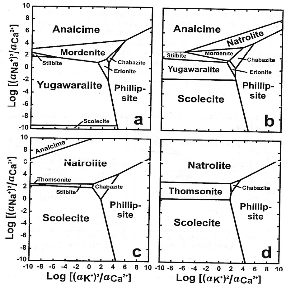
Figure 10. \log[(aK^+)^2/aCa^{2+}] vs. \log[(aNa^+)^2/aCa^{2+}] diagrams for the zeolites occurring in vugs and cavities in mafic volcanic rocks (analcime, chabazite, erionite, heulandite, laumontite, mesolite, mordenite, natrolite, phillipsite, scolecite, stilbite, thomsonite, and yugawaralite) calculated assuming 35°C and (a) \log a(SiO_2) = -4.0 ; (b) \log a(SiO_2) = -4.1 ; (c) \log a(SiO_2) = -4.3 ; (d) \log a(SiO_2) = -5.0 .
