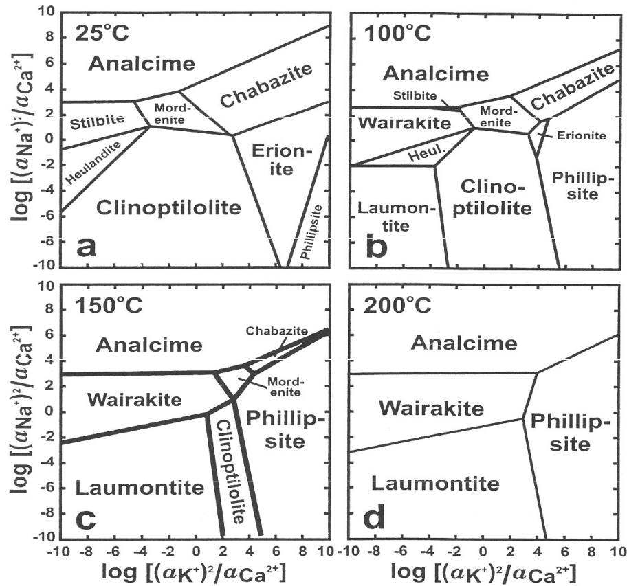
Figure 9. \log[(aK^+)^2/aCa^{2+}] vs. \log[(aNa^+)^2/aCa^{2+}] diagrams for zeolites occurring in hydrothermal deposits in silicic-volcanic rocks (analcime, chabazite, clinoptilolite, erionite, heulandite, laumontite, mordenite, phillipsite, stilbite, and wairakite), all calculated assuming an aqueous silica activity in equilibrium with quartz and at (a): 25°C, (b): 100°C, (c): 150°C, (d): 200°C.
