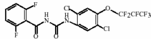
lufenuron
