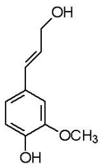
Coniferyl alcohol
