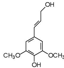
Sinapyl alcohol
