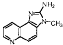
IQ
