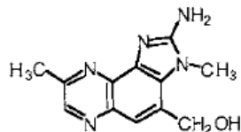
4-CH 2 OH-8-MeIQx
