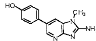
4'-hydroxy-PhIP
