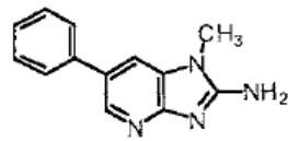
PhIP
