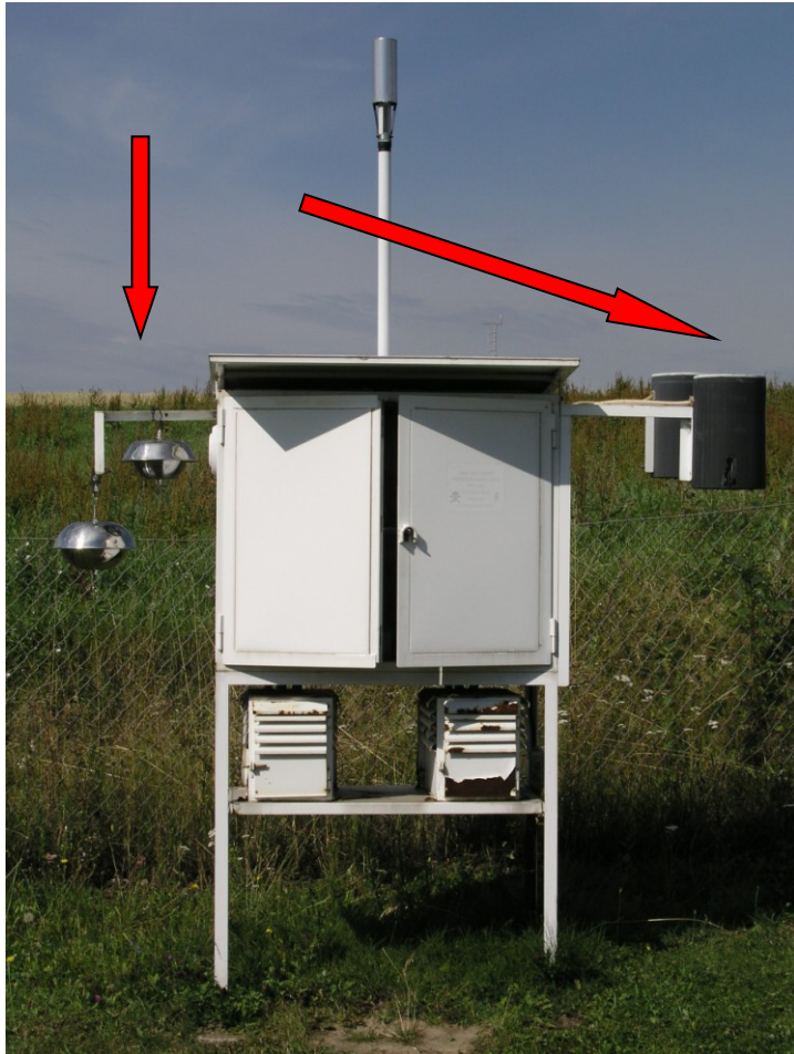
passive samplers
