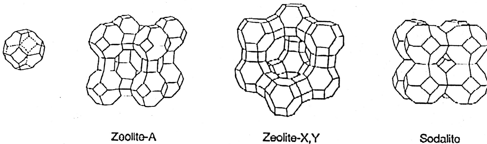
Figure 2. The sodalite cage (left), and the structures of zeolite A, zeolite X/Y, and sodalite 9 .
