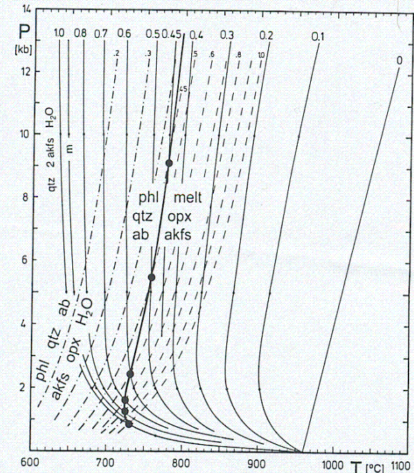
Fig. 9.5. Pressure-temperature diagram for parts of the system \text{K}_2\text{O-SiO}_2\text{-Al}_2\text{O}_3\text{-MgO-H}_2\text{O} , showing the relationship between subsolidus dehydration equilibrium curves, beginning of melting curves and solidus for dehydration melting of phlogopite-quartz-albite assemblages. Dash-dotted curves Equilibrium curves of the a_{\text{H}_2\text{O}} -controlled dehydration reaction: phlogopite + quartz + albite = alkali feldspar + orthopyroxene + \text{H}_2\text{O} ; continuous curves solidus curves for given a_{\text{H}_2\text{O}} of the haplogranite system (as in Fig. 2.13); dots and heavy continuous curve solidus for the dehydration melting reaction: phlogopite + quartz + albite = akfs + orthopyroxene + melt; dashed curves metastable portions of the dehydration reaction. Abbreviations as in Appendix
