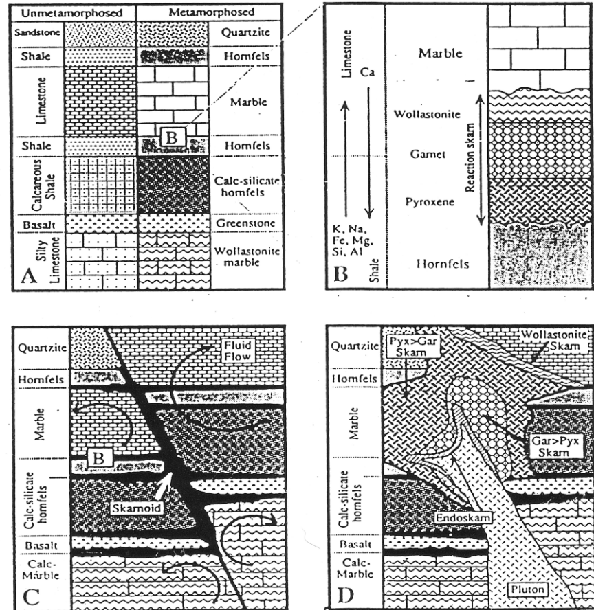
Figure 1 Types of skarn formation: (A) Isochemical metamorphism involves recrystallization and changes in mineral stability without significant mass transfer; (B) Reaction skarn results from metamorphism of interlayered lithologies, such as shale and limestone, with mass transfer between layers on a small scale (bimetasomatism); (C) Skarnoid results from metamorphism of impure lithologies with some mass transfer by small-scale fluid movement; (D) Fluid-controlled metasomatic skarn typically is coarse grained and does not closely reflect the composition or texture of the protolith.
