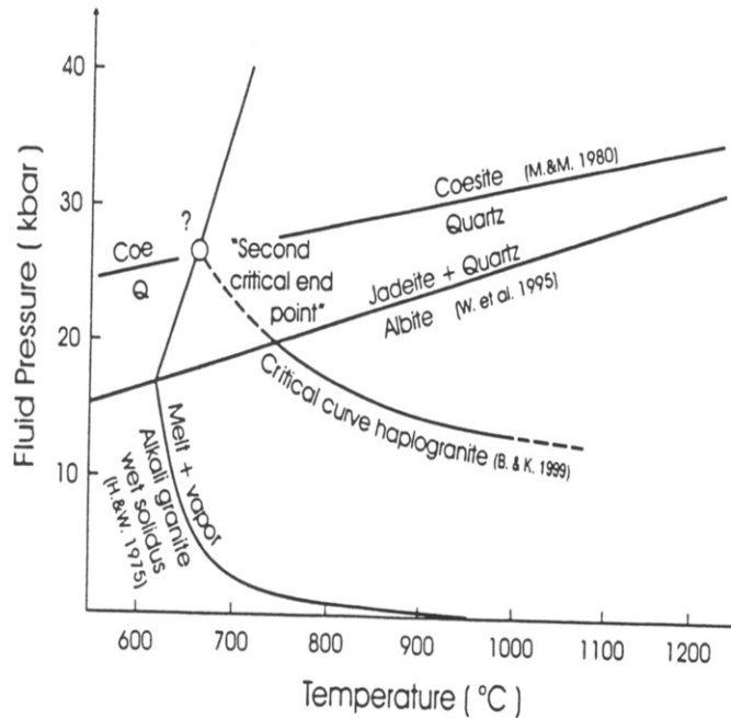
FIG. 3. Pressure-temperature plot showing the critical curve of a haplogranite as determined by Bureau and Keppler (1999), together with other relevant reaction curves. Upper pressure stability limits of albite are after Waterwiese et al. (1995) and of quartz after Mirwald and Massonne (1980); the "wet melting curve" of an alkali granite was taken from Huang and Wyllie (1975). Note that the latter curve is intersected by the extrapolated critical curve (dashed line). However, because of the larger number of components present in this system, the resulting point cannot be compared directly with the second critical end point shown in Figure 1 for albite-water. Nevertheless, supercritical behavior of a more complex nature takes place at higher pressures, and the "wet melting curve" of Huang and Wyllie (1975) should no longer be present there.
