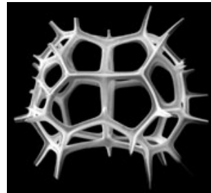
Lophospyris pentagona
