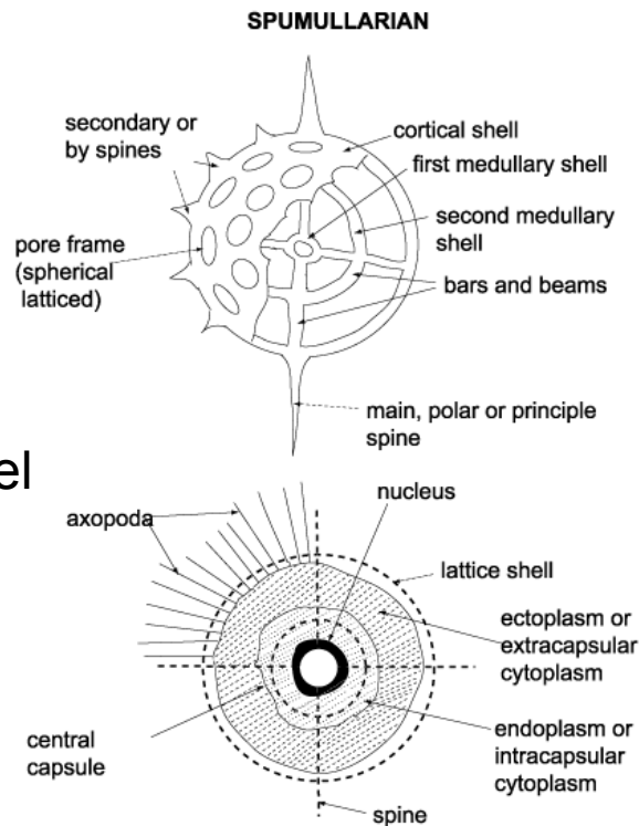
Diagrammatic cross-sections of spumullarian radiolaria.
