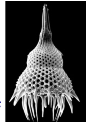
Lamprocyclas maritilis
