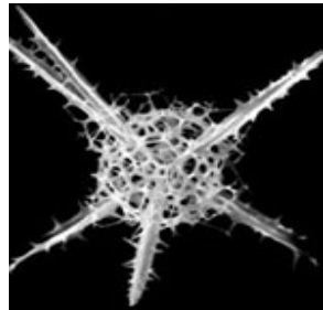
Rhizophlegma boreale
