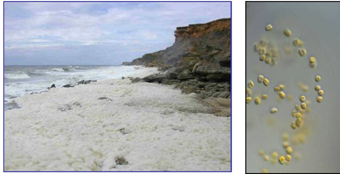
Phaeocystis sp.
