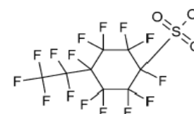
Perfluorinated cyclo sulfonates (ex. PFECHS)
