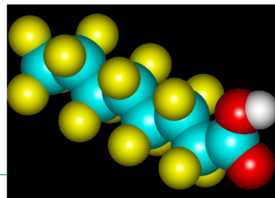
Perfluorooctanoic acid (PFOA)
