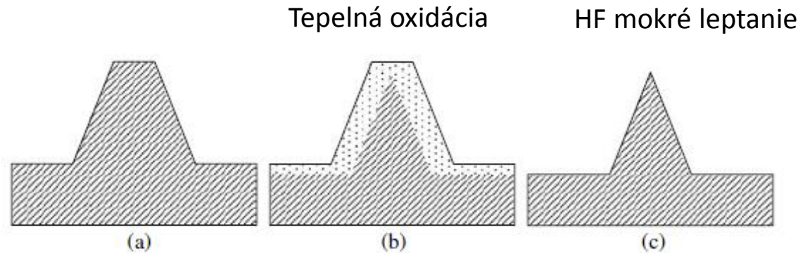
Fig. 7.9 Schematic of oxidation sharpening process. (a) Initial tip geometry, (b) oxidation, (c) final tip geometry after removal of oxide layer
