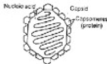
icosahedral nucleocapsid
