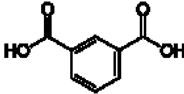
isophthalic acid
