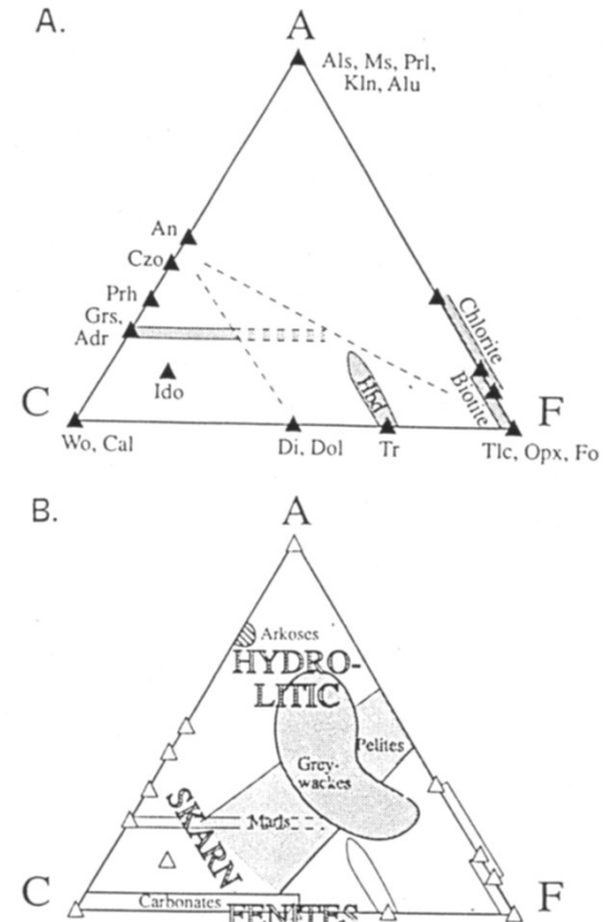
Figure 1. ACF projection of minerals and generalized rock compositions commonly involved in metasomatic aureoles. A. Mineral compositions. B. Generalized fresh rock compositions and schematic regions for metasomatic types.
