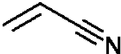
AKRYLONITRIL
