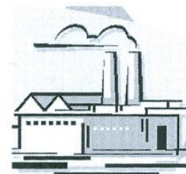
Atmospheric deposition
