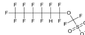
Polyfluorinated ether sulfonates (ex. Perfluoro [hexyl ethyl ether sulfonate])
