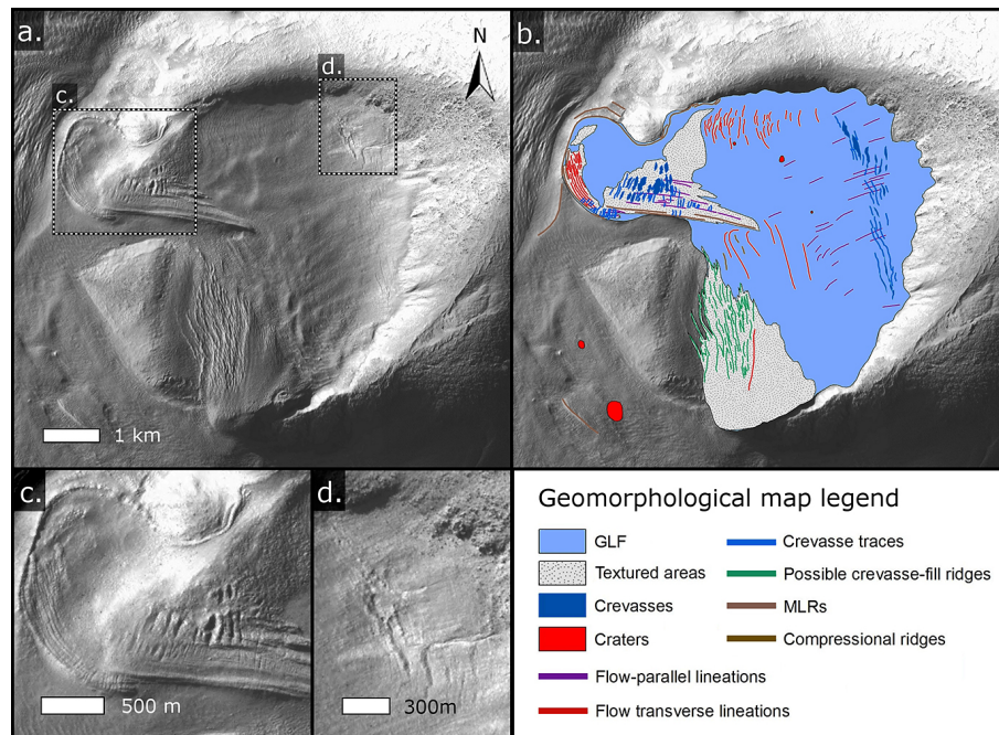
Figure 6. CTX image of crevassed GLF #1054, located in eastern Hellas (Fig. 5a) (a), along with its geomorphological interpretation (b) and expansions of two crevasse sets (c and d).
