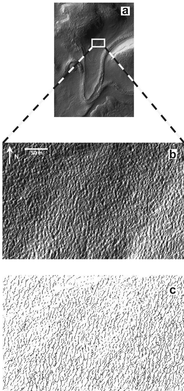
Figure 10. Surface incisions on GLF #947 imaged by HiRISE to supplement those reported on GLF #948 by Hubbard et al. (2011). GLF #947 (a) with an expansion of the incised terrain (b) and trace of incised segments (c).
