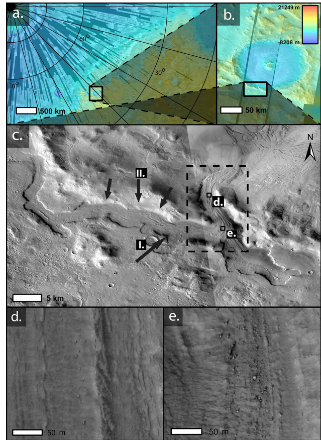
Figure 8. HiRISE image of GLF #498, located in Protonilus Mensae showing background MOLA elevation images (a and b), and an expansion of GLF #498 (c), along with two examples of surface boulder exposures (d and e). Arrows I. and II. on panel (c) indicate likely source areas for supra-GLF boulders illustrated in Fig. 9 and discussed in the text. The dashed box is expanded in Fig. 9.
