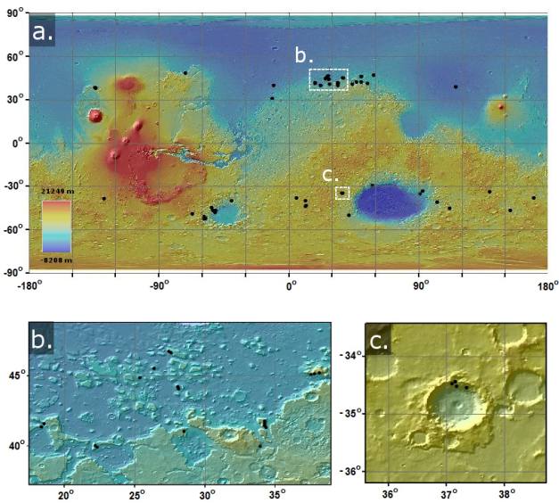
Figure 5. The distribution of crevassed GLFs on Mars (a), with expansions of GLF clusters in Deuteronilus Mensae (b) and western Hellas Planitia (c).
